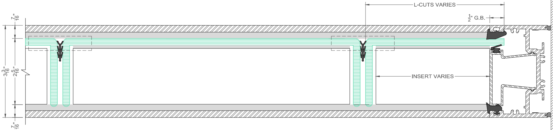
1 JAMB DETAIL WITH FULL CHANNELS SD-3 SCALE: 6" = 1'-0"
