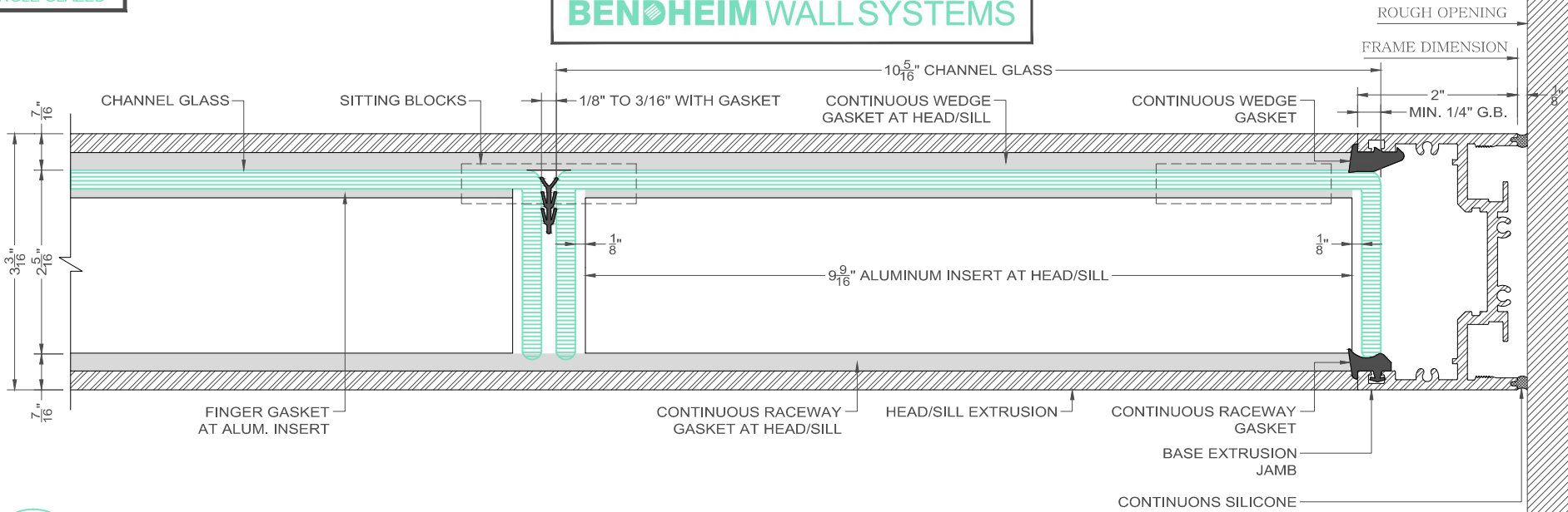
1 JAMB DETAIL WITH FULL CHANNELS SD-3 SCALE: 6" = 1'-0"
