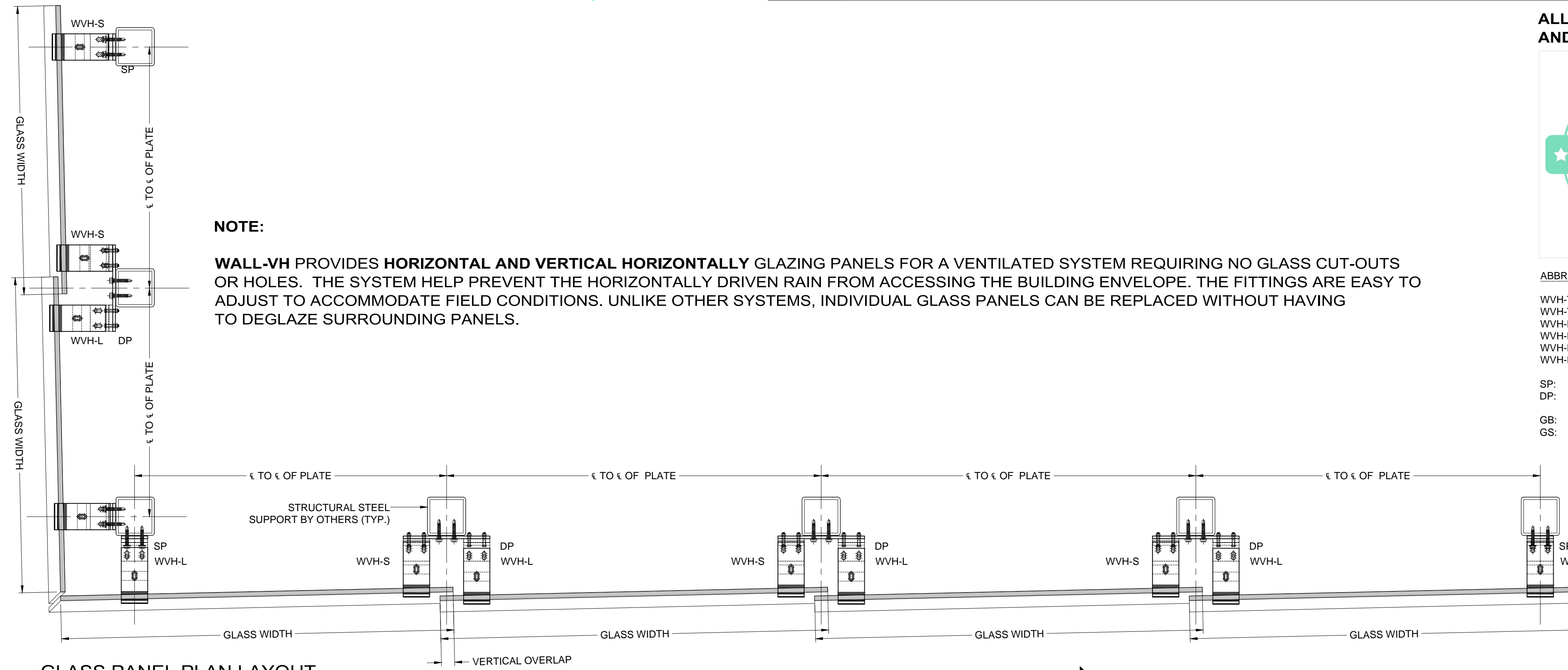
GLASS PANEL PLAN LAYOUT
