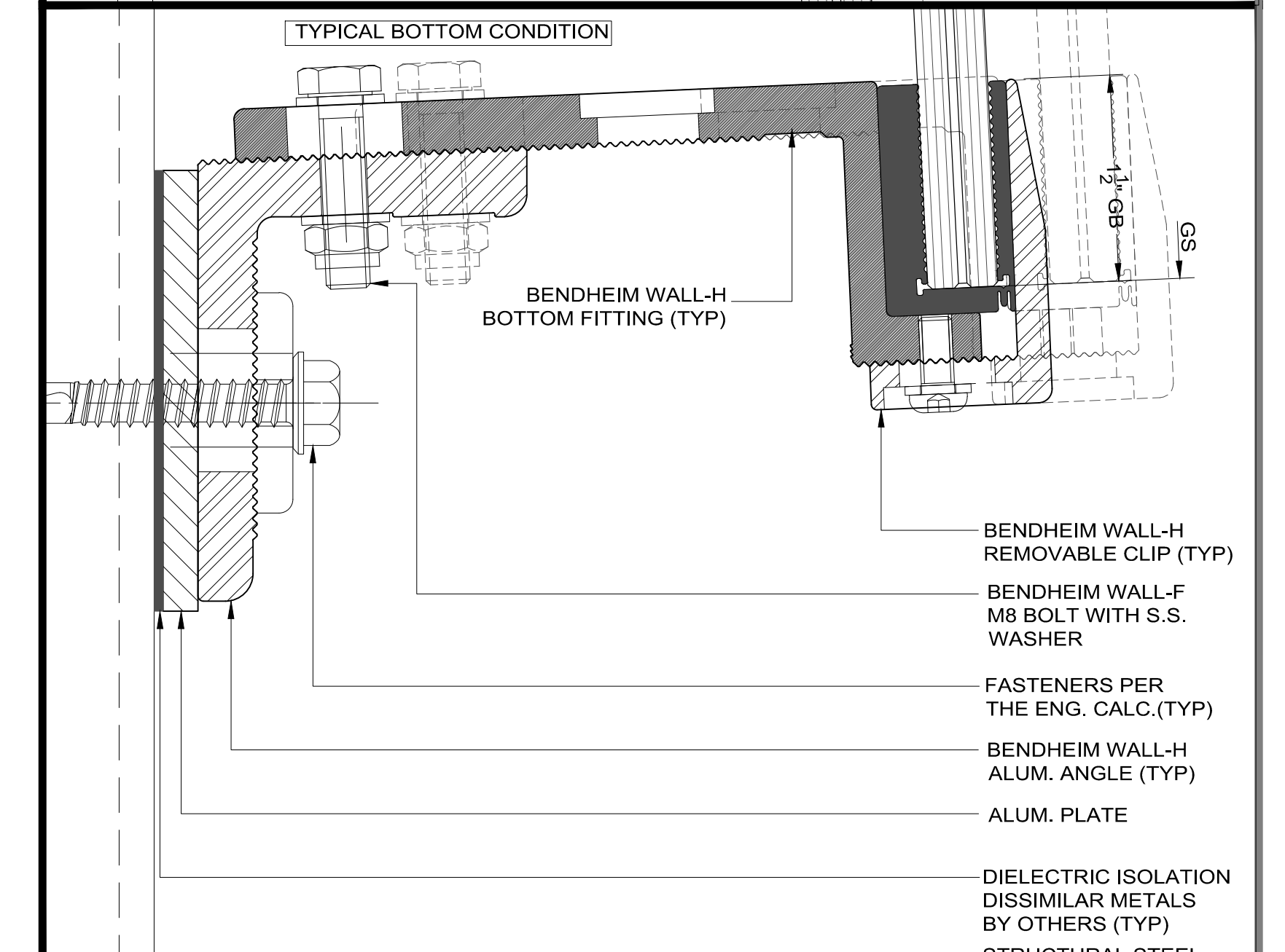
DETAIL "D-D"
