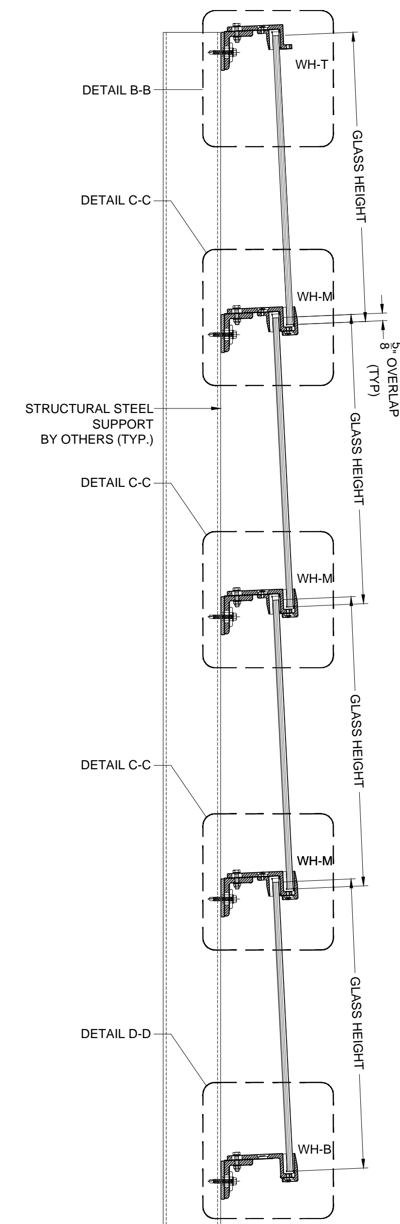
SECTION "A-A"
