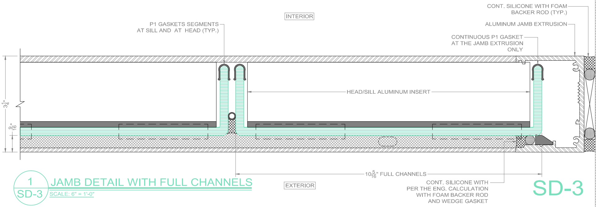
1 JAMB DETAIL WITH L-CUTS SD-3 SCALE: 6" = 1'-0"
